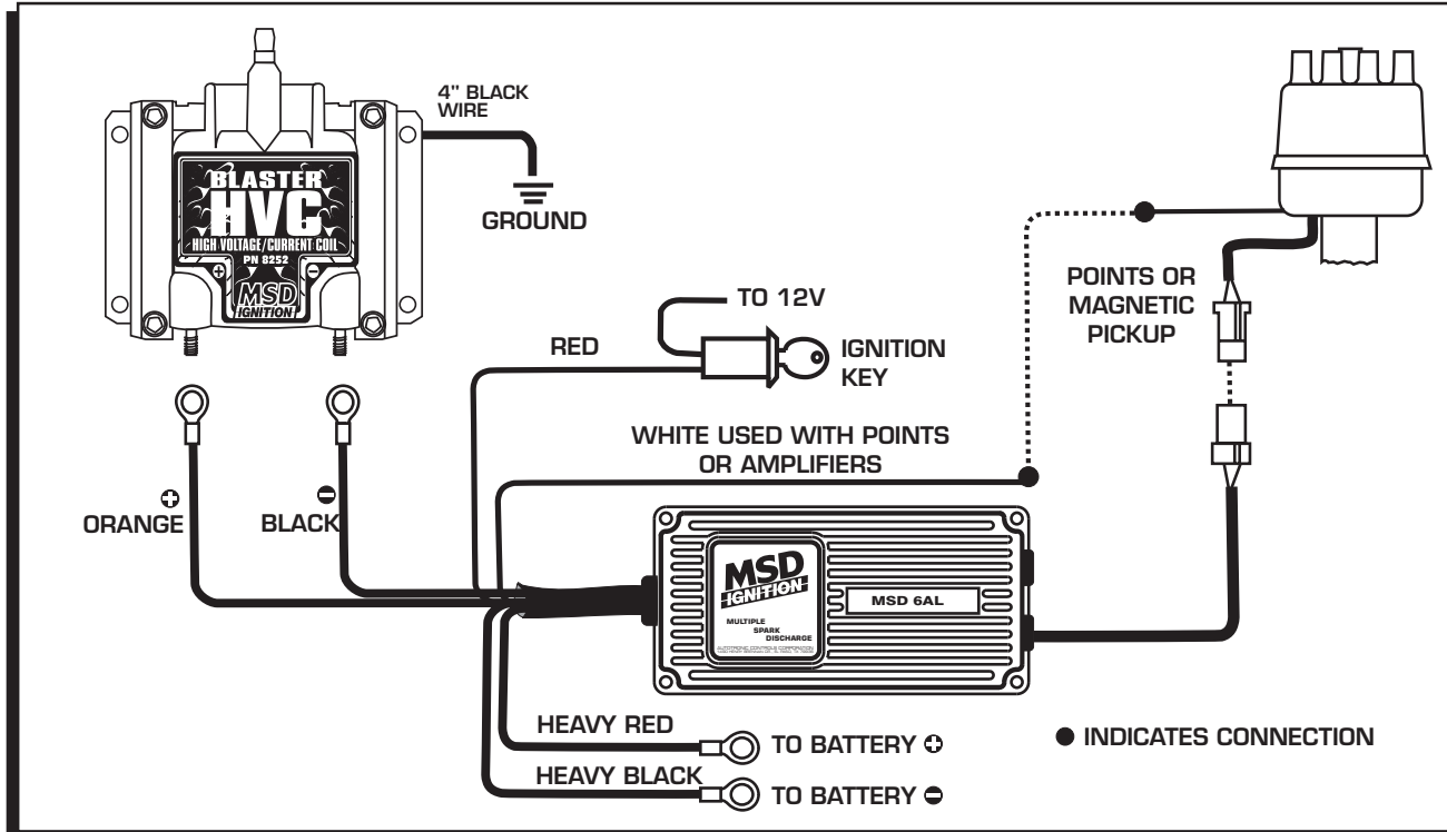
Wiring to an MSD 6 Series Ignition.
